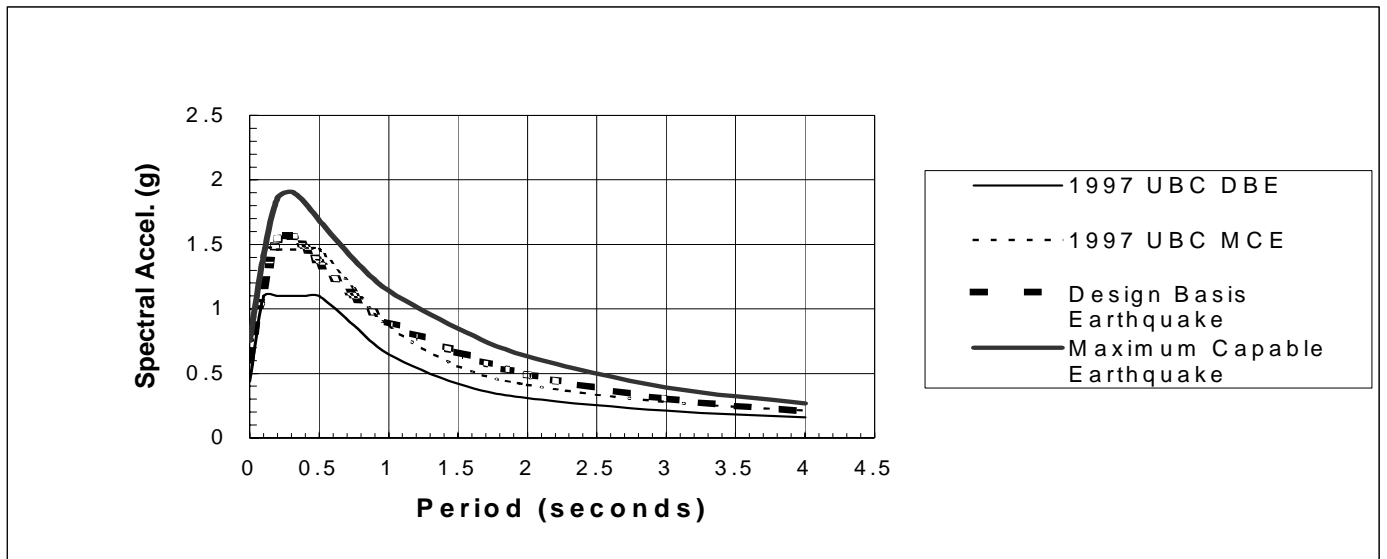
Figure 3. Response spectra graphs for 5% damped structures.
