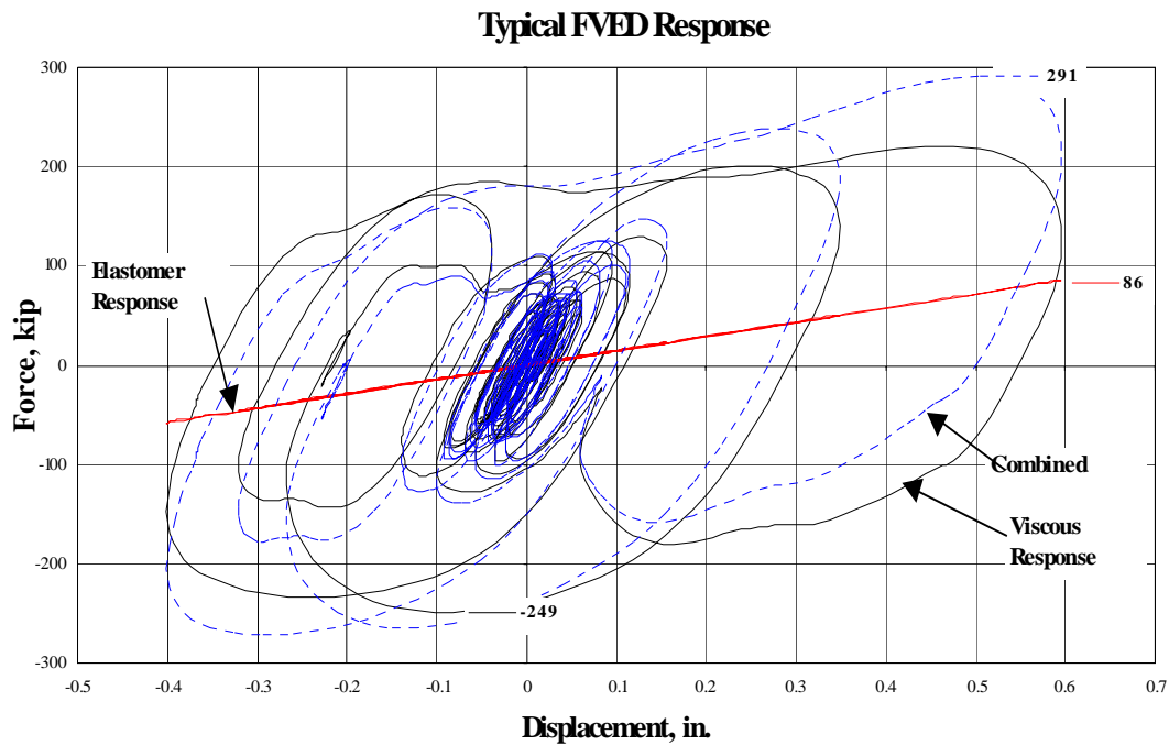
Figure 15: Typical FVED response
