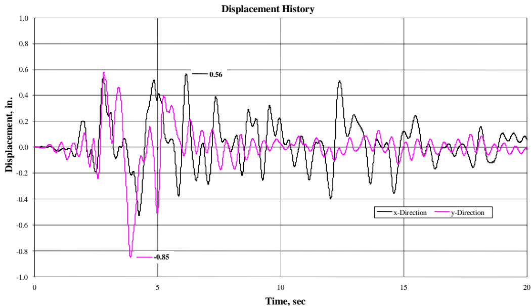
Figure 14: Displacement History of Damped Structure
