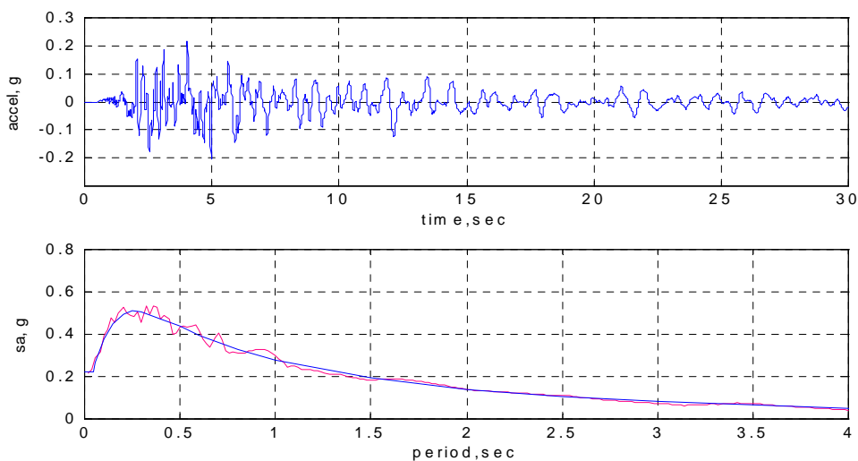
Figure 5: Acceleration Record & Spectrum
