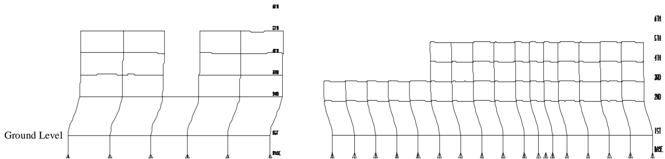
Figure 6: Modes 1 & 2 (Elevations)
