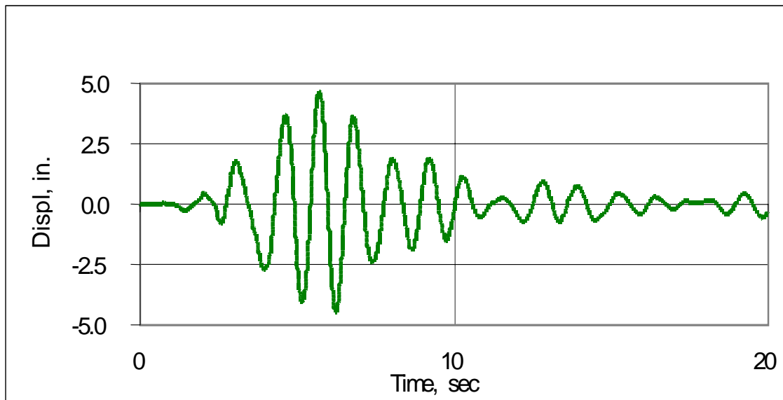
Figure 11: Displacement History of Existing Structure (Linear Model)
