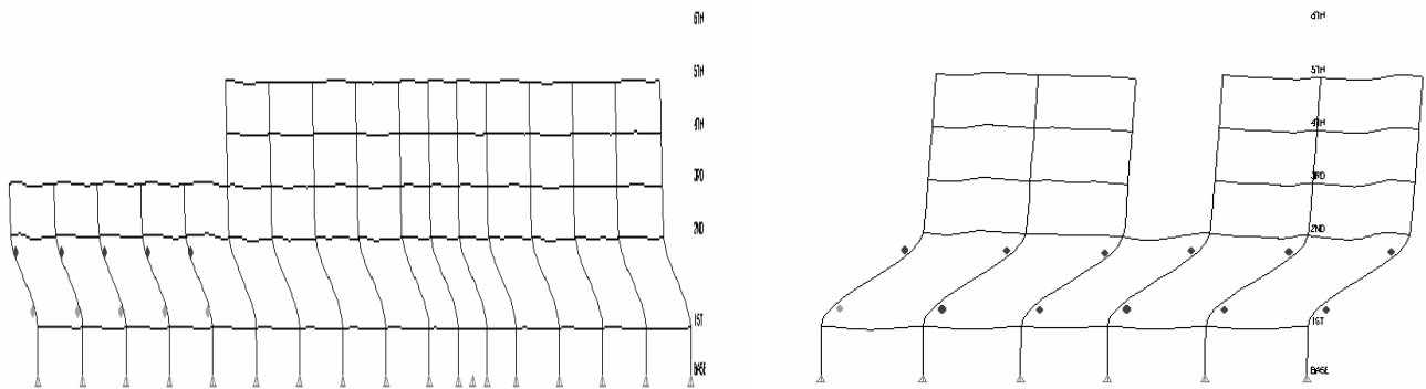
Figure 9a & 9b: Progressive Hinge Formation (elevations)
