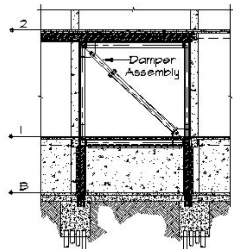
Figure 12: Damper Frame Elevation
