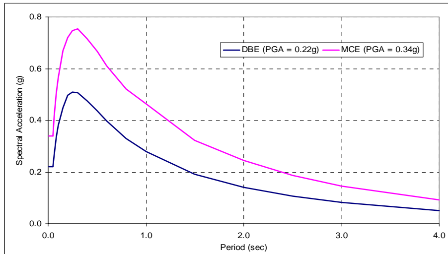
Figure 4: Response Spectra
