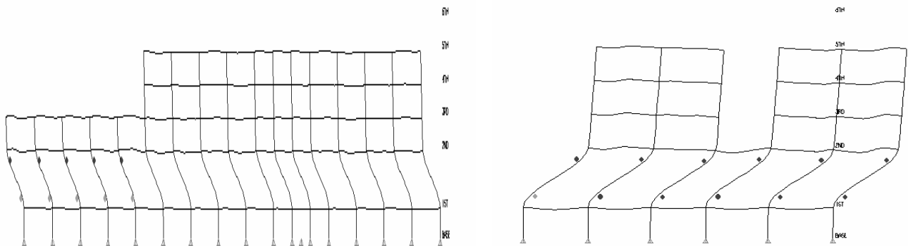
Figure 9a & 9b: Progressive Hinge Formation (elevations)
